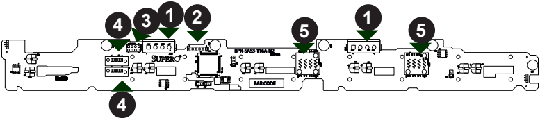
Figure 2-1. Rear Connector Locations
