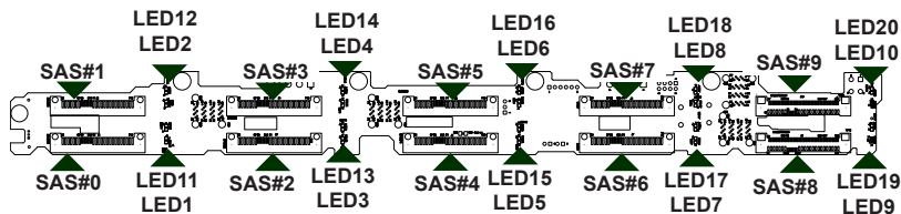
Figure 2-3. Front Connectors and LEDs
