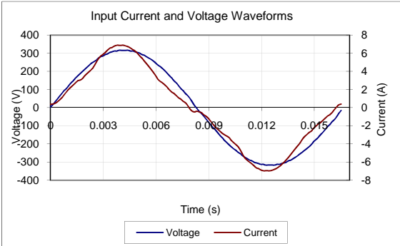
Input AC Current Waveform (ITHD = 20.45%, 50% Load)
