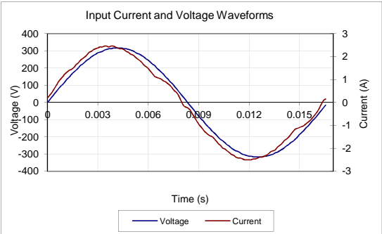
Input AC Current Waveform (ITHD = 5.34%, 50% Load)
